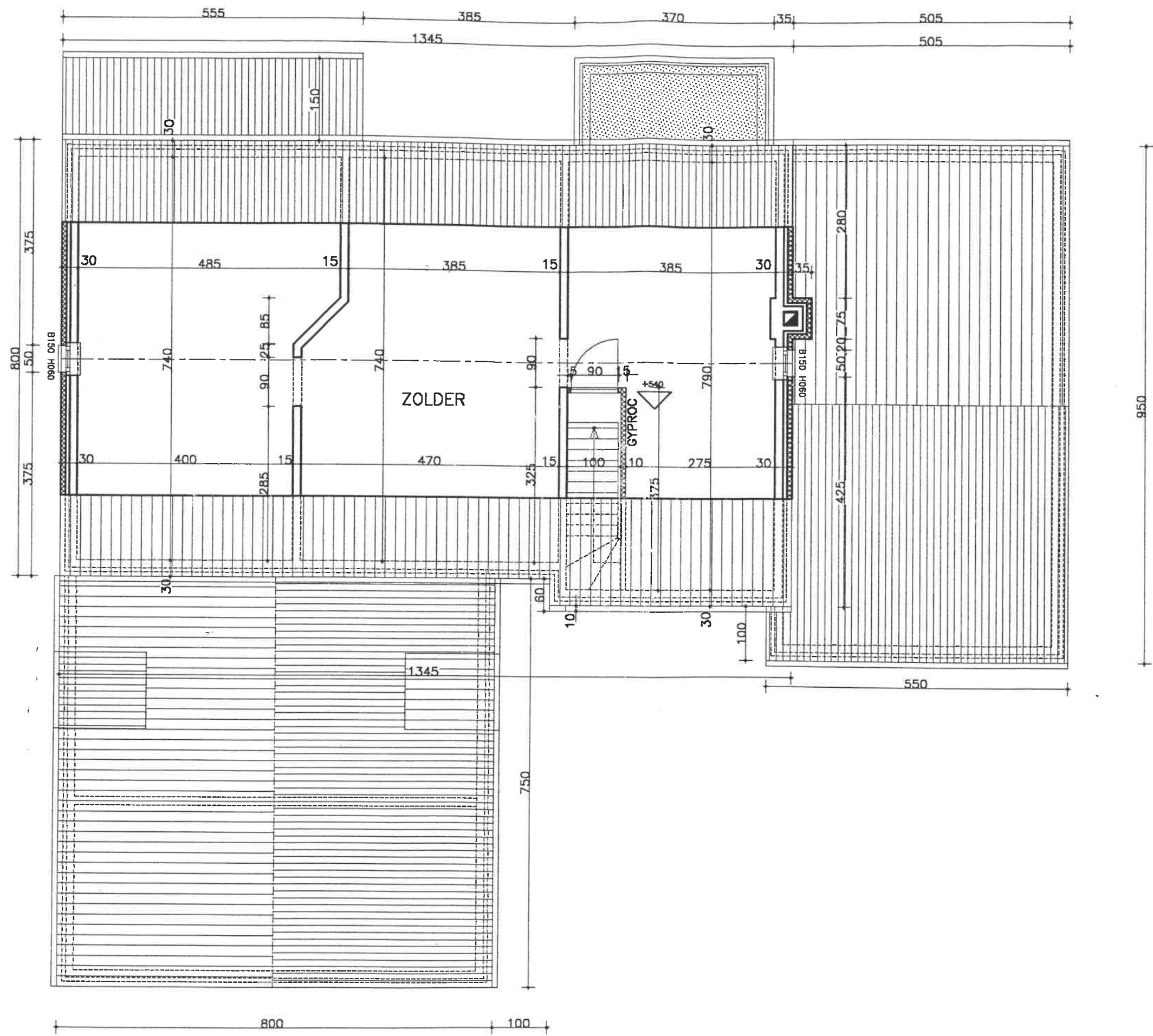
ZOLDERPLAN sch. 1/75
