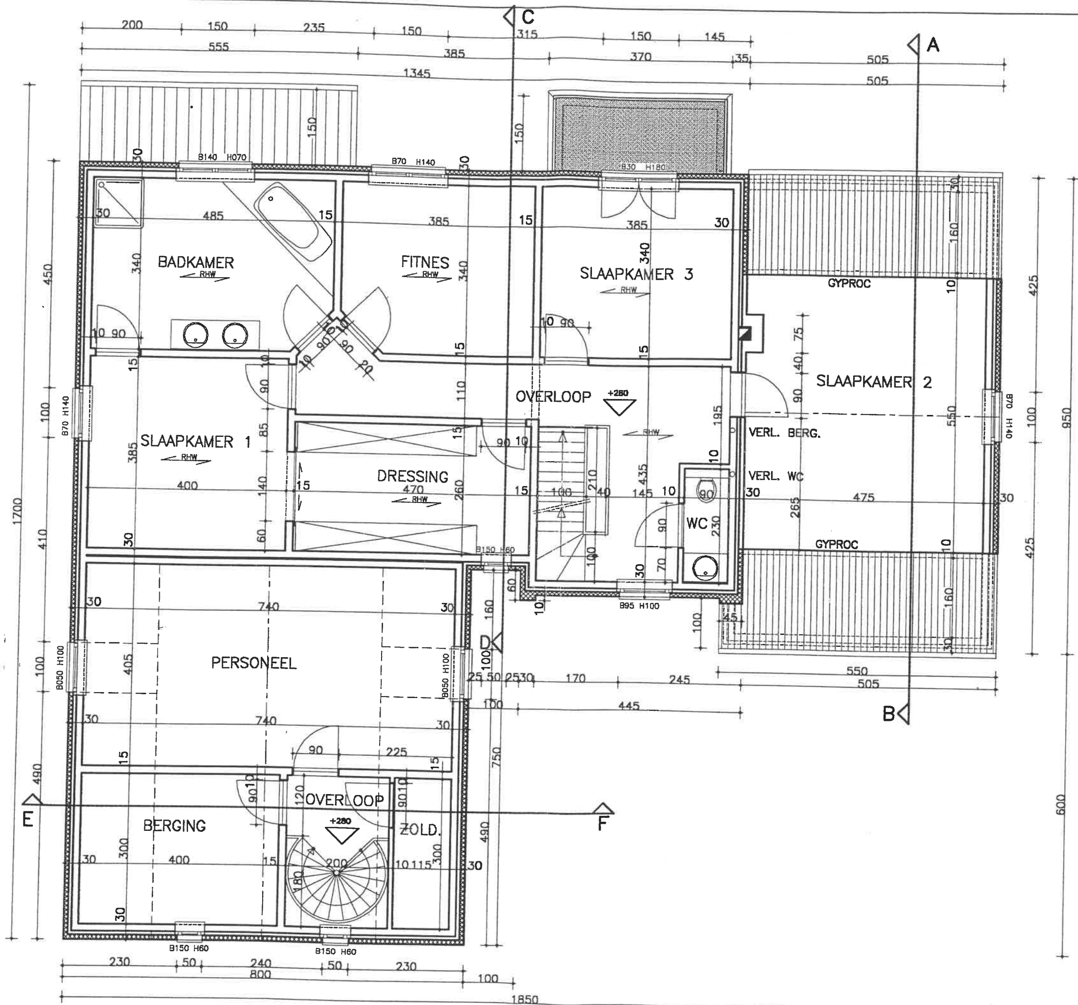
VERDIEPINGSPLAN sch. 1/75
