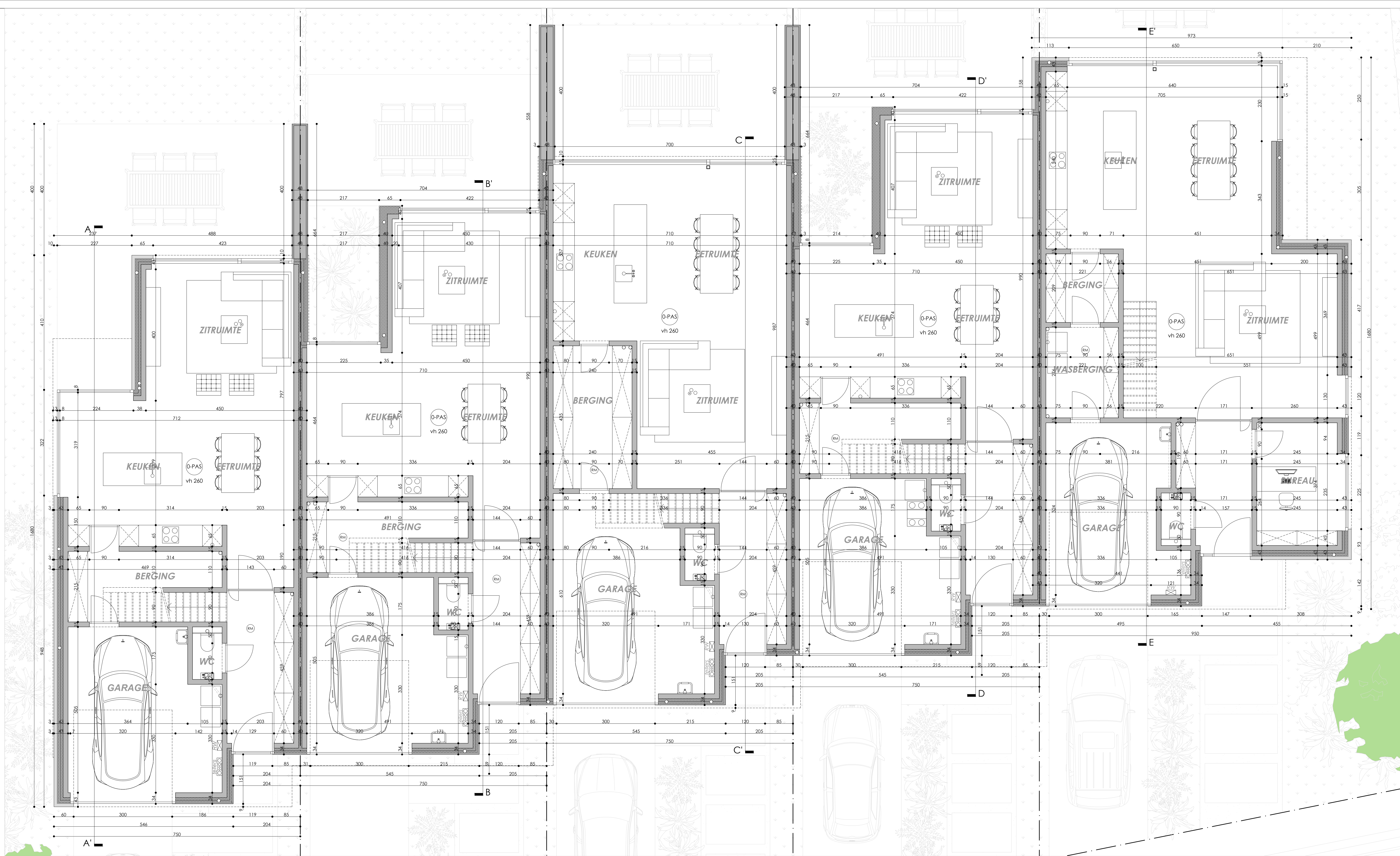
PLAN 0
