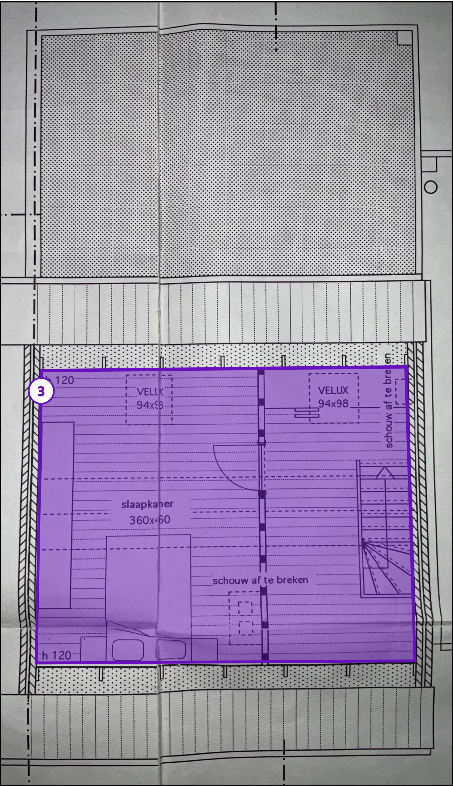
Legende van plan 1.7: Zolder - plafonds in hout
