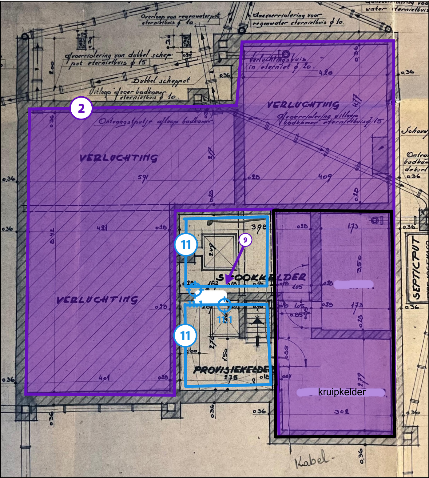
Legende van plan 1.1: Woning plan kelder
