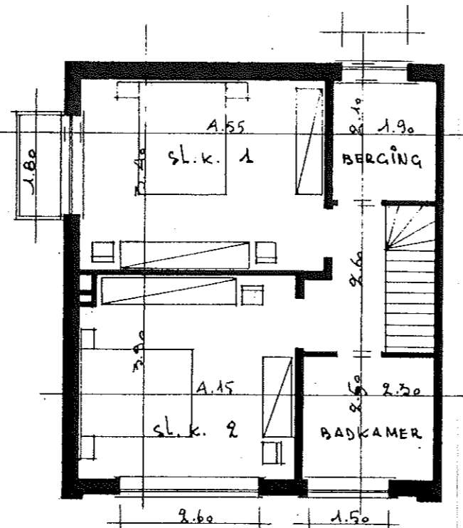
VERDIEPING.
