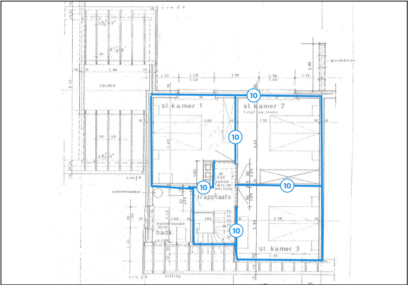
Legende van plan 1.11: Plan verdieping
