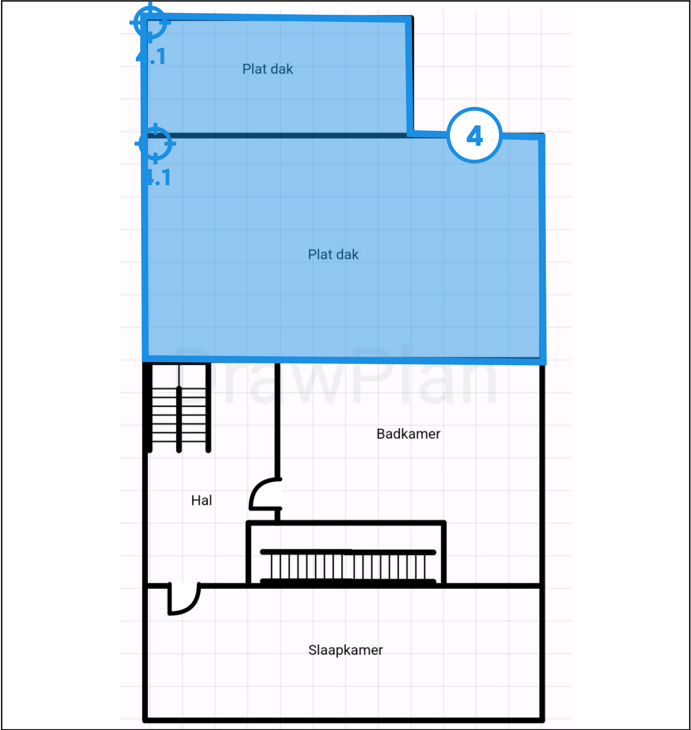
Legende van plan 1.10: Verdiep +1 : roofing plat dak
