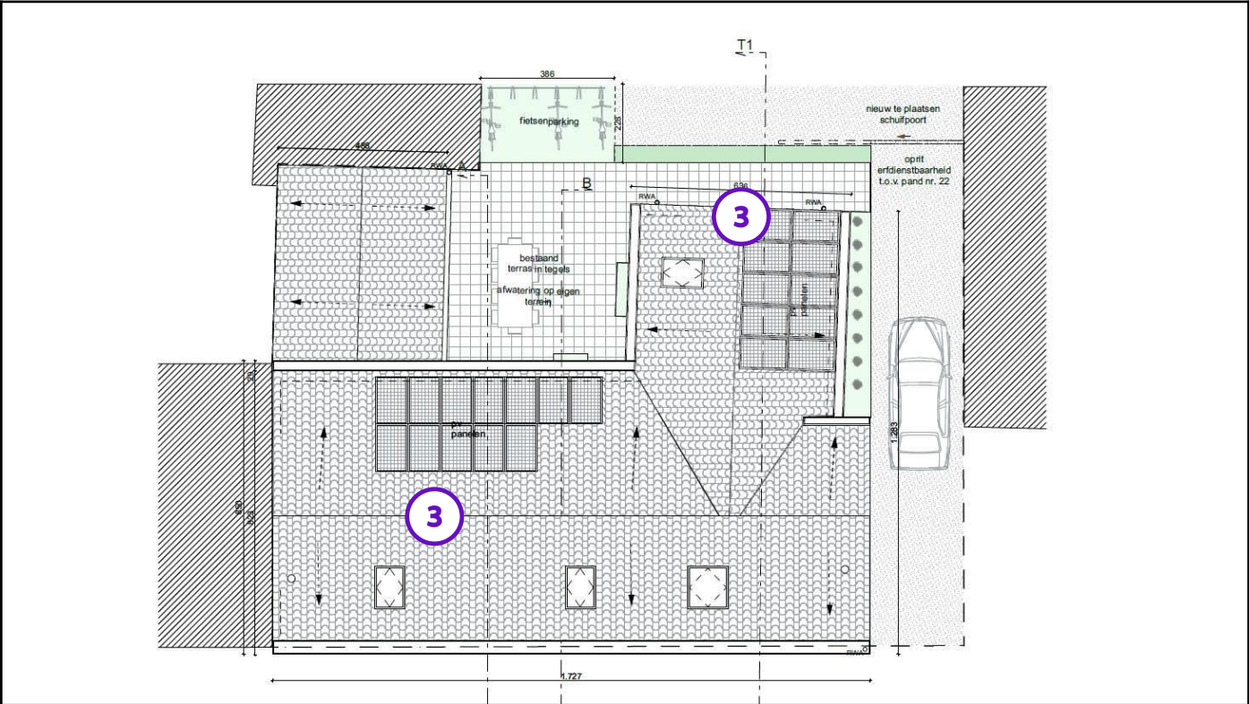
Legende van plan 1.8: Plan dak
