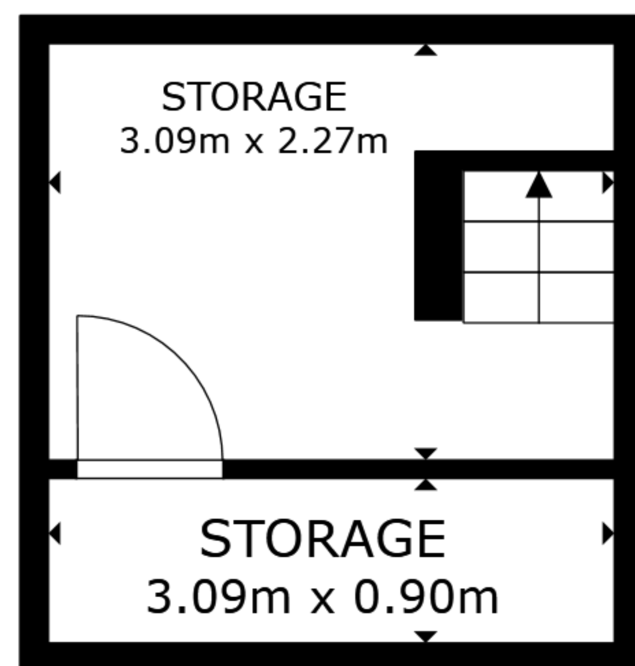
FLOOR 1
