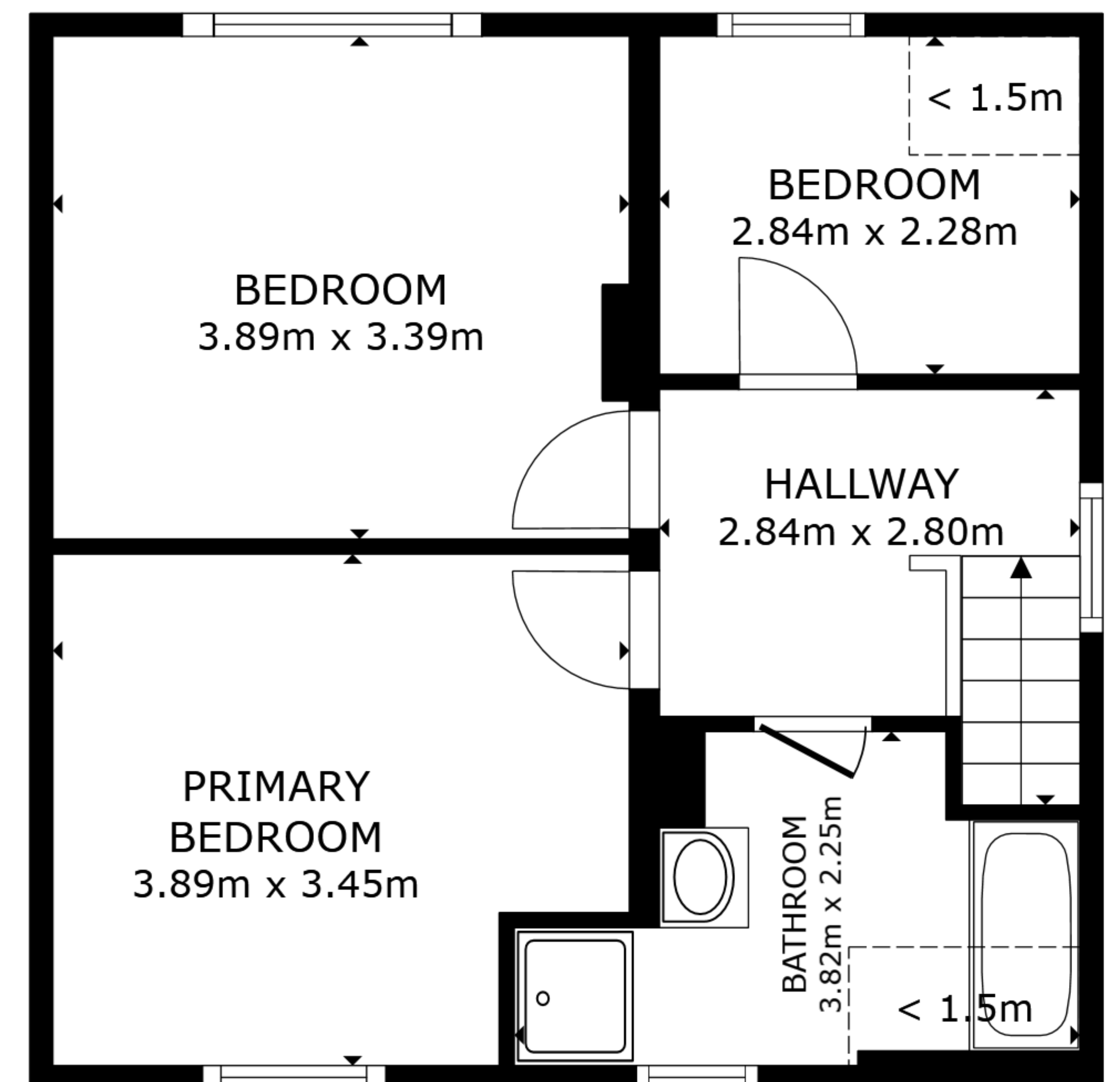
FLOOR 3
